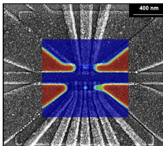
The electron density inside a silicon quantum device.
