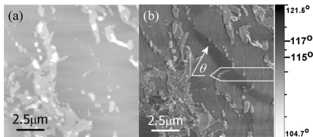
(a) Topography of a poly(diacetylene) film. Regions of monolayer, bilayer, and trilayer are visible. (b) Simultaneously acquired phase image. The gray-scale variations through the center of the film correspond to variations in in-plane shear and friction as measured by tapping mode AFM.
